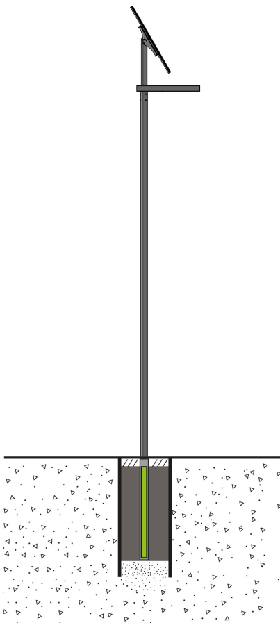
BUISFUNDERING
