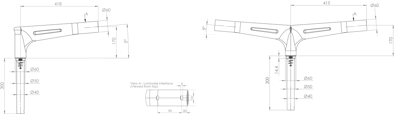
DRILLING INFORMATION FOR LATERAL MOUNTING ON POLE
