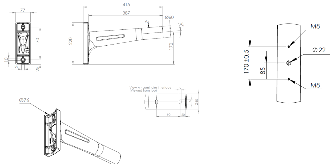
DIO LATERAL & WALL S415
